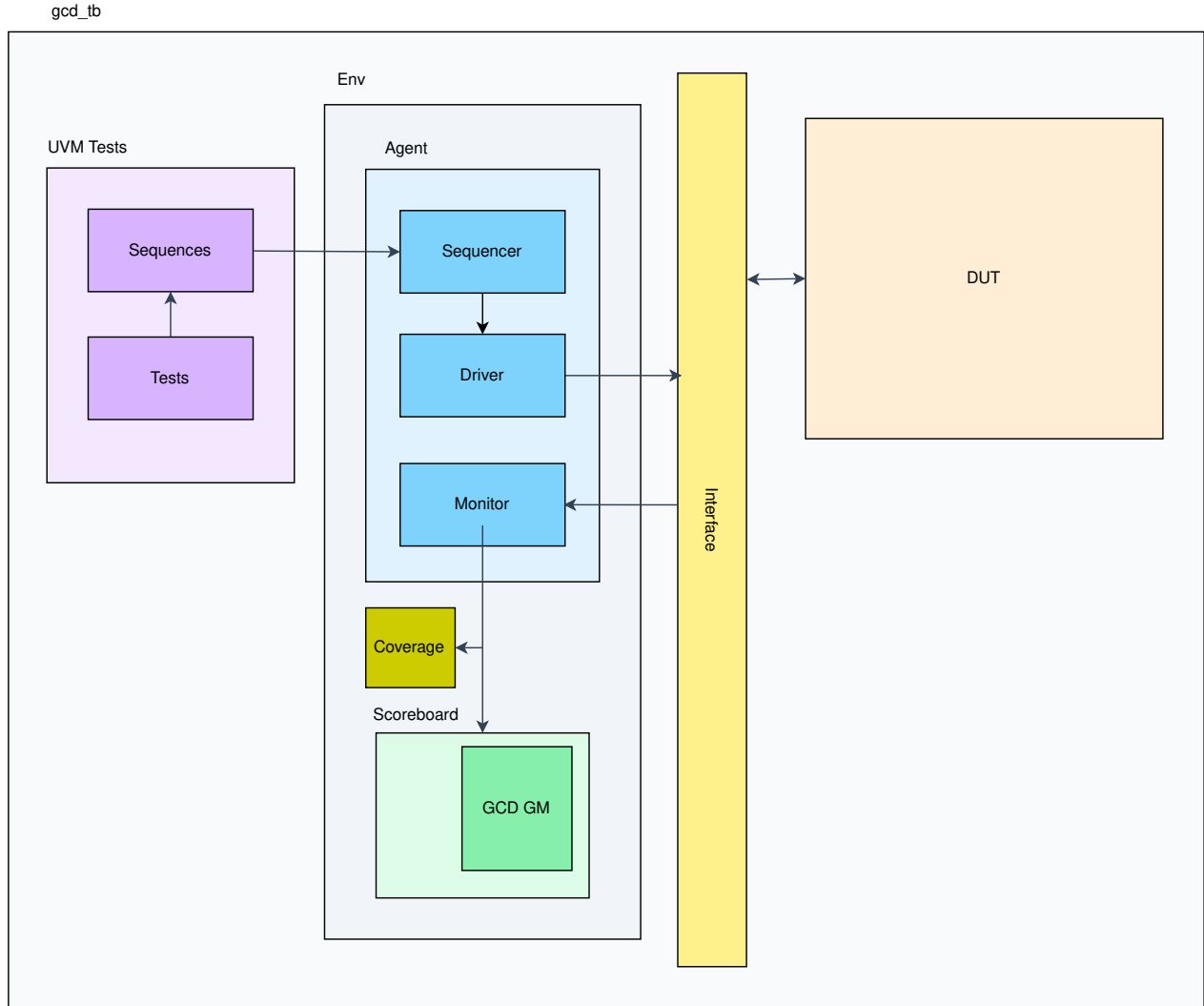
Figure 1: UVM testbench architecture diagram
